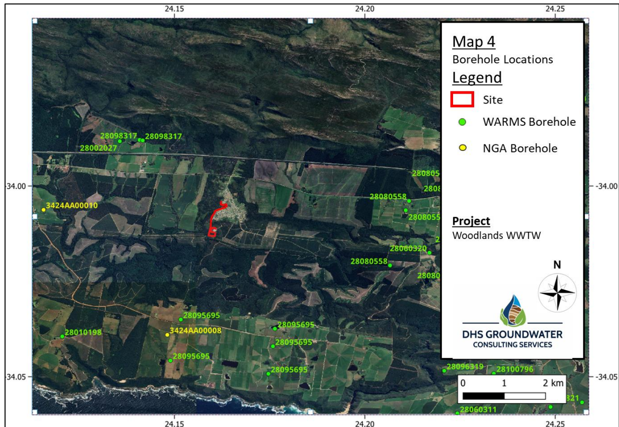
Figure 7. Borehole locations.
